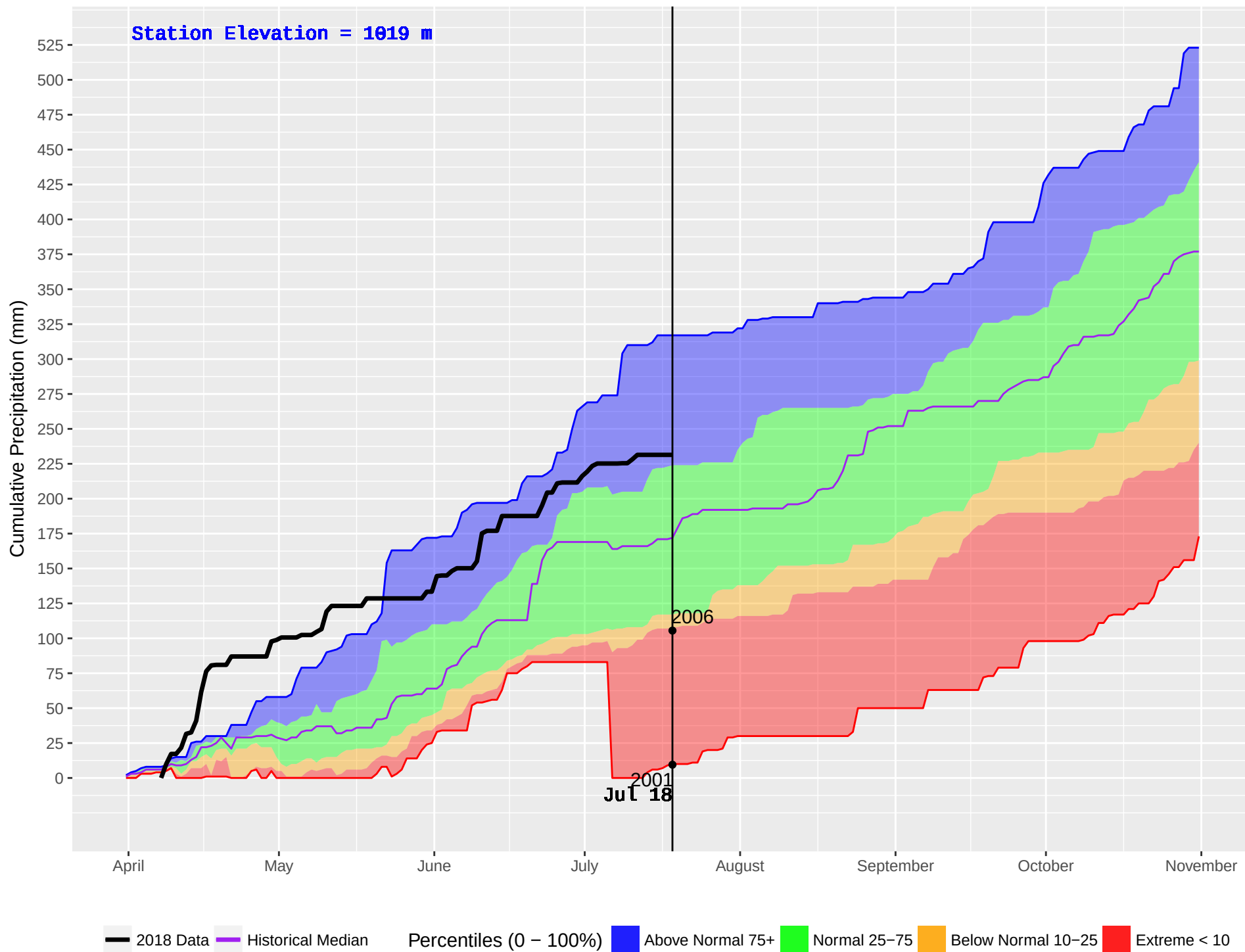
POWDER CREEK (380) : Historical (2001–2016) and Current (2018) Daily Cumulative Precipitation
