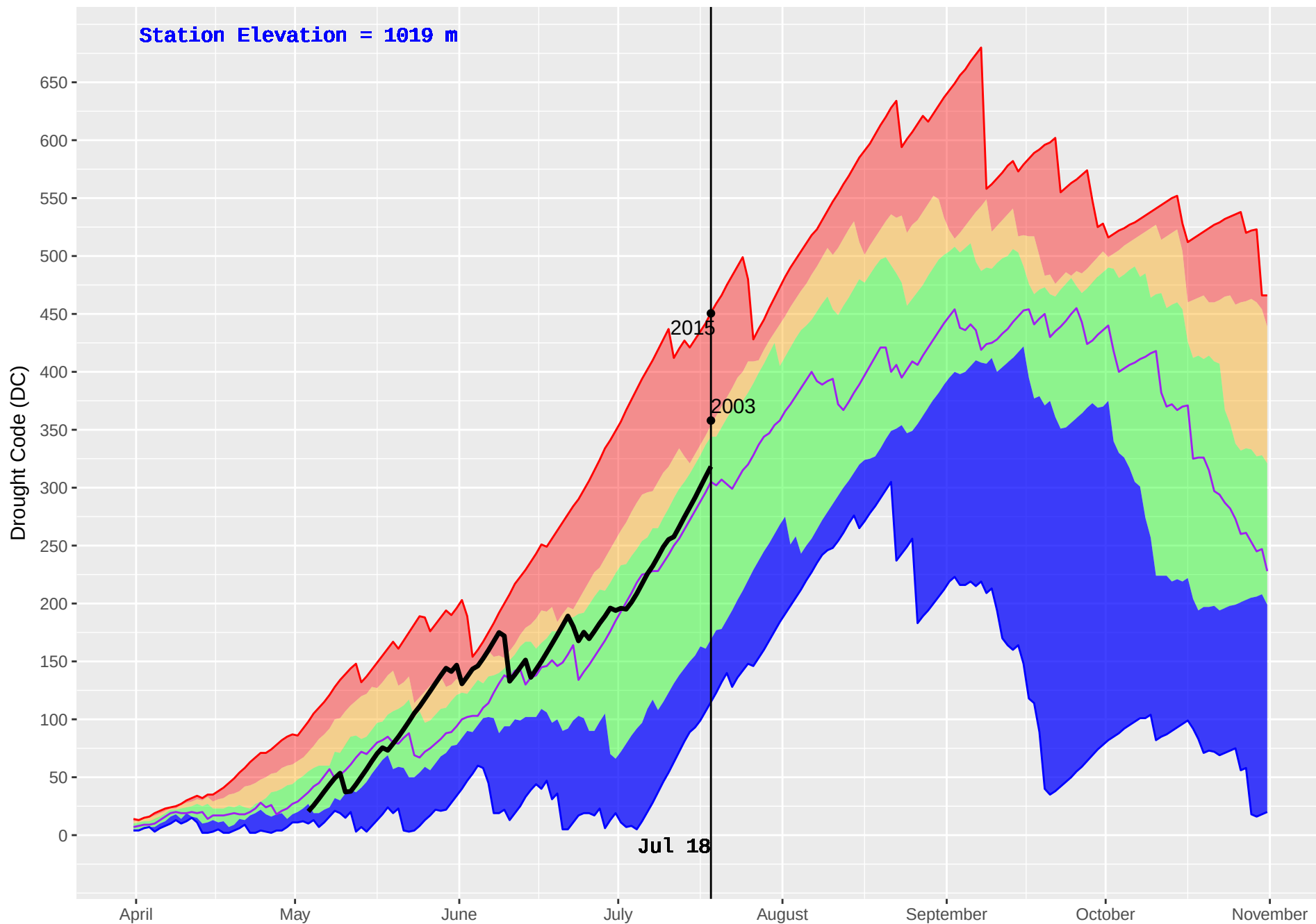
POWDER CREEK (380) : Historical (2001–2016) and Current (2018) Daily Drought Code (DC)
