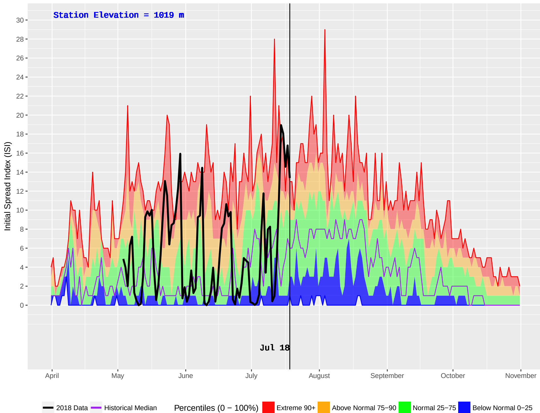
POWDER CREEK (380) : Historical (2001–2016) and Current (2018) Daily Initial Spread Index (ISI)
